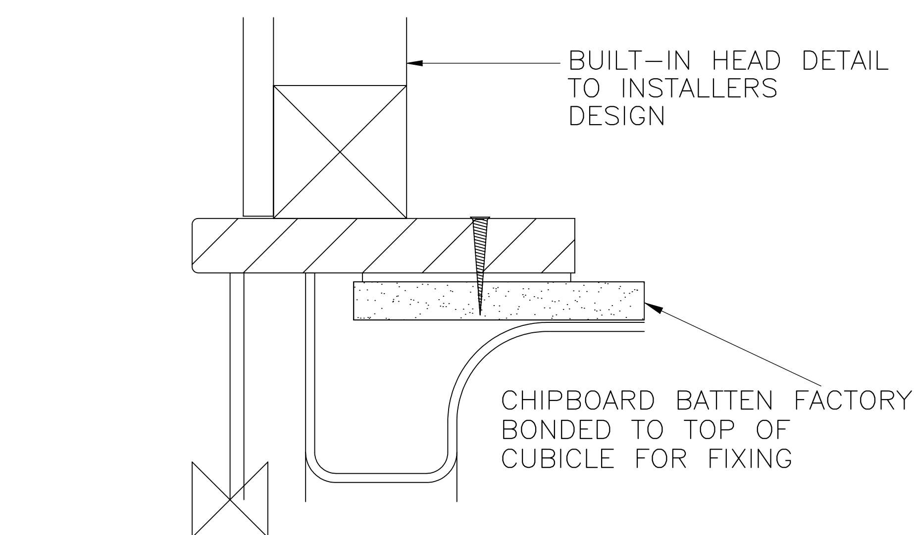
DETAIL B SUGGESTED SECTION THROUGH HEAD OF SHOWER CUBICLE
