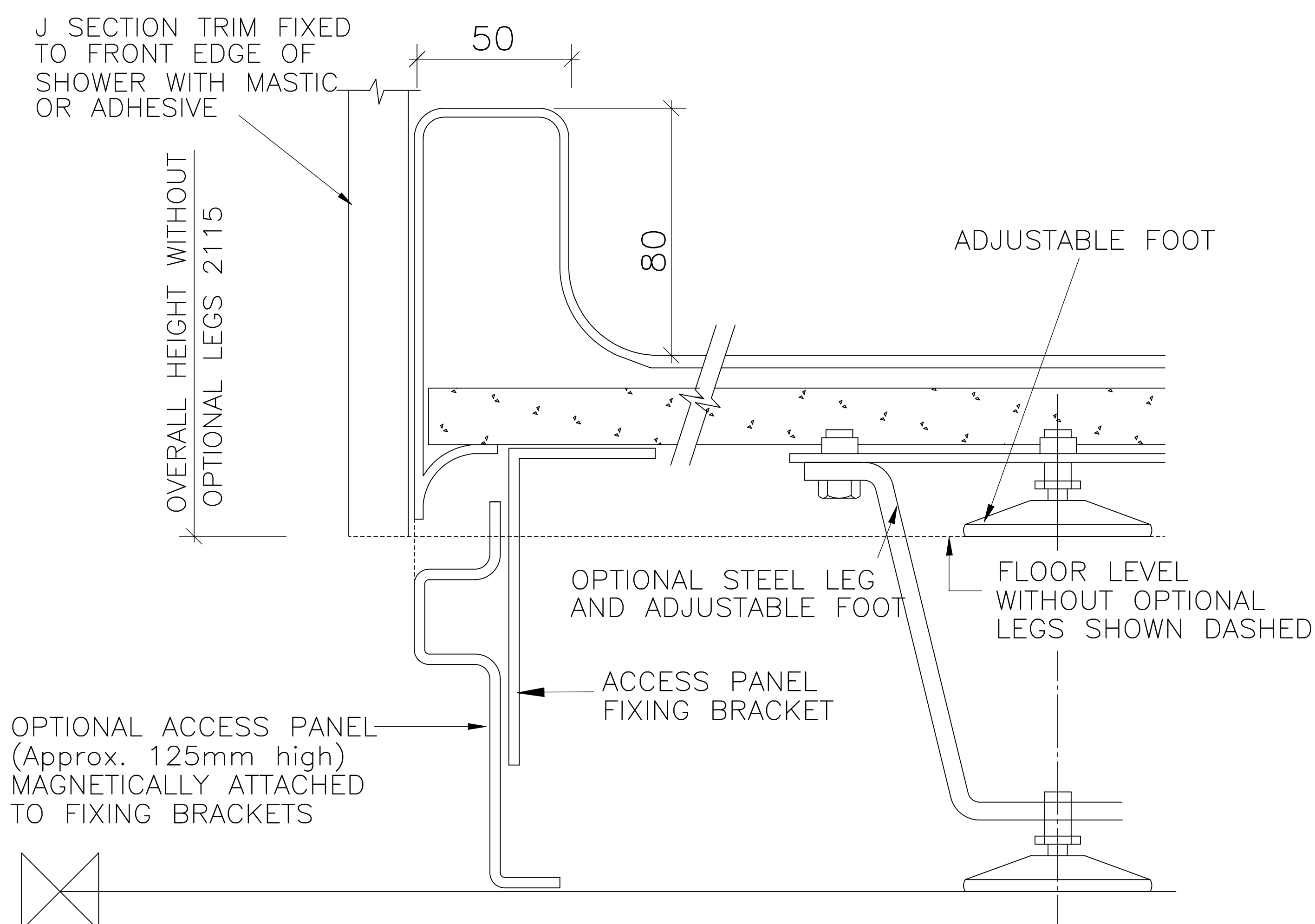
DETAIL A SECTION THROUGH THRESHOLD & ACCESS PANEL
