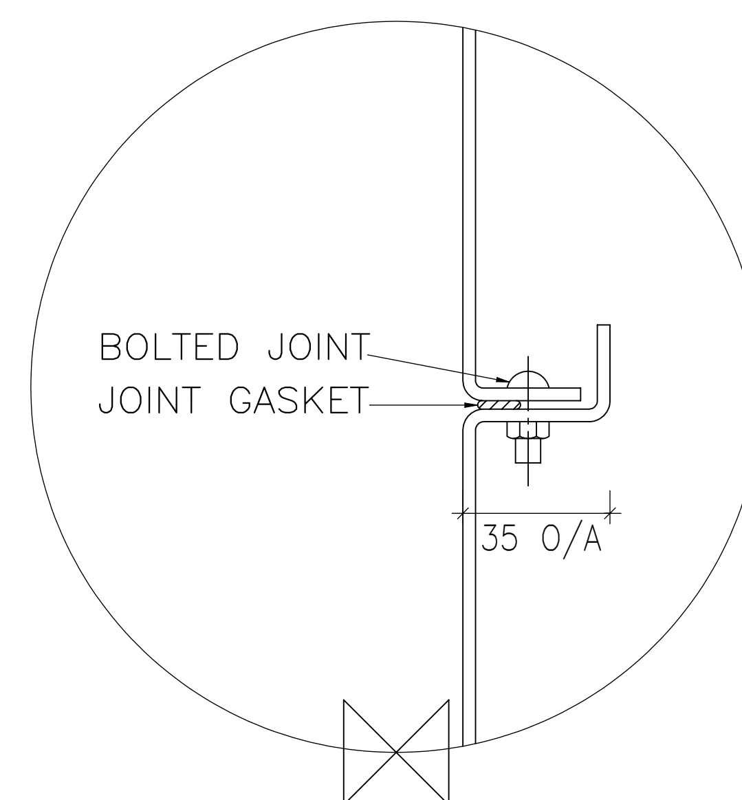
DETAIL C VERTICAL SECTION THROUGH JOINT
