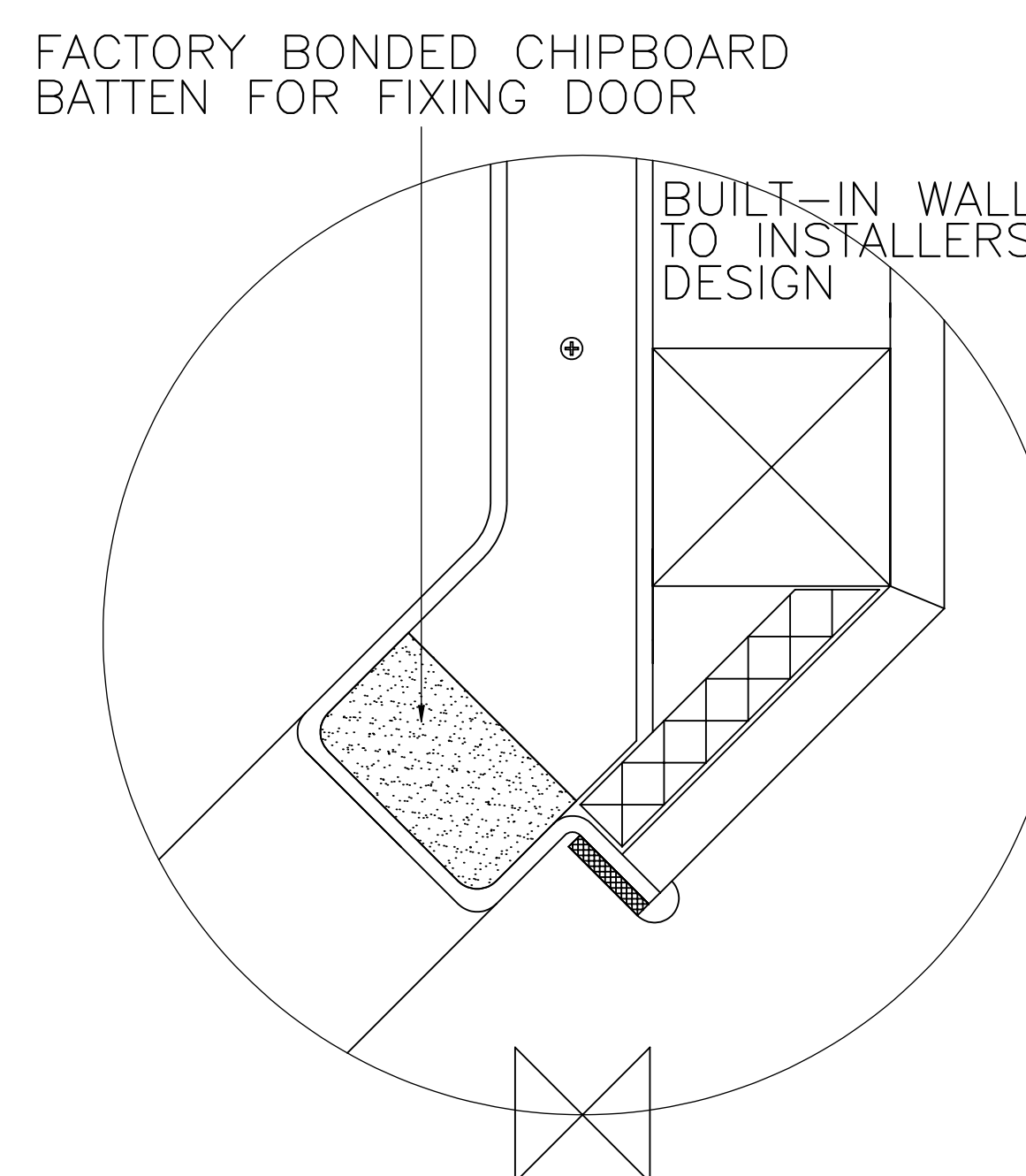
DETAIL D SECTION THROUGH DOOR FRAME
